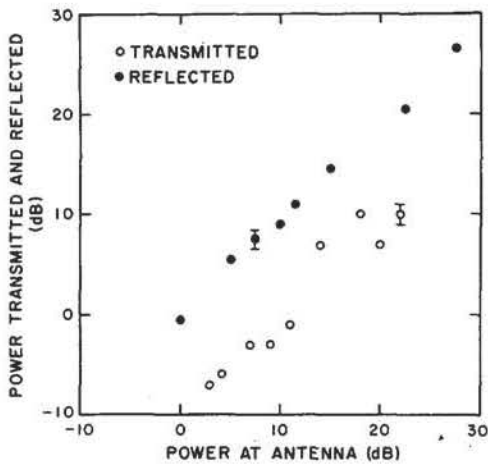
FIG. 1. Lower-hybrid wave power reflected by or transmitted through the grid as a function of wave power approaching the grid. Wave frequency, 30 MHz. Here 0 dB corresponds to 29 mW delivered to wave launching antenna.
