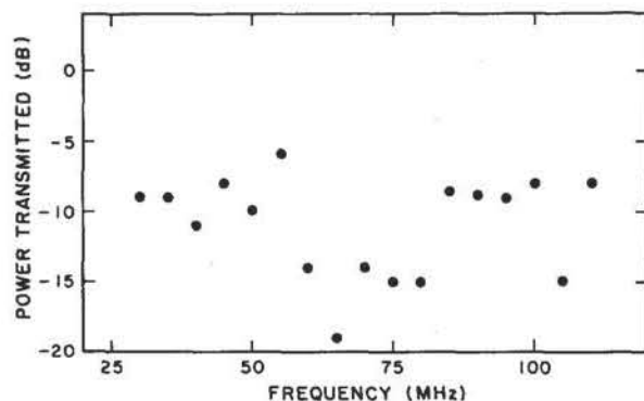
FIG. 2. Lower-hybrid wave power transmitted through grid, compared to wave power approaching grid, versus wave frequency.
